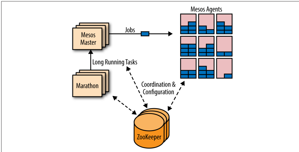
Figure 12-4. Mesos cluster
